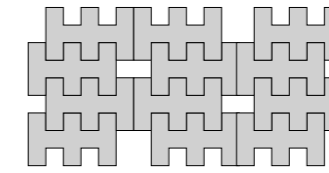
schema posa 2 laying scheme 2 42 pcs / sqm
