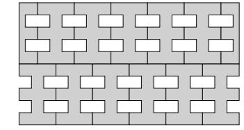
schema posa 3 laying scheme 3 35 pcs / sqm
