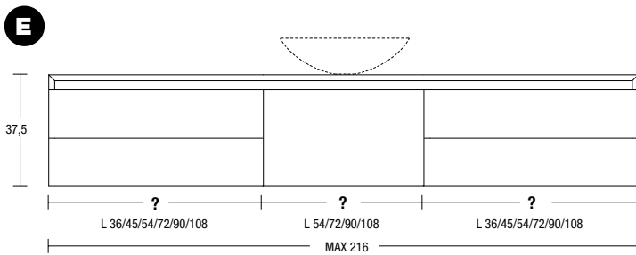
Base con 2 cassetti Double drawer cabinet
