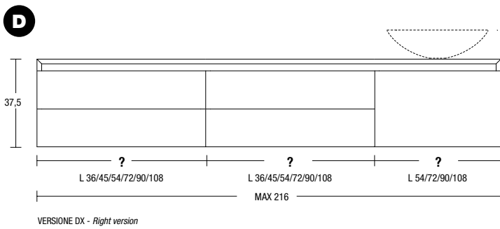
Base con 2 cassetti Double drawer cabinet
