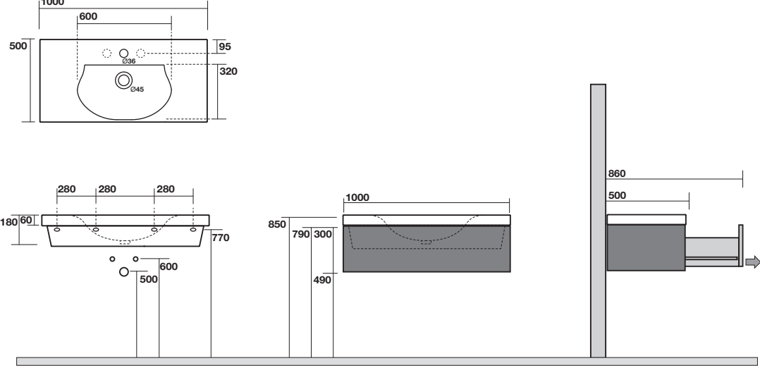
3937 Lavabo 100x50 monoforo (3 fori a richiesta) per mobile sospeso One hole washbasin 100x50 (3 holes on demand ) for cabinet 9175 Mobile sospeso in legno 100x50X30 per lavabo sospeso Wooden draw unit for washbasin 100x50X30
