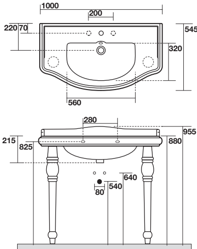
7300 Struttura porta lavabo 100 in ottone con gambe coniche e ripiano in griglia Metal structure with conic legs and shelf for washbasin 100
