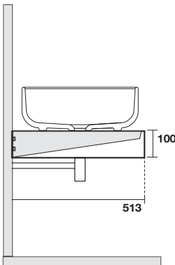
7335 Mensola sospesa cm 120 Wall hung shelf cm 120
