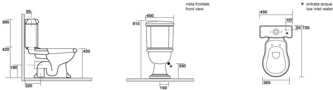
1012 vaso monoblocco scarico suolo “S” Close couped wc pan floor outlet 1013 vaso monoblocco scarico parete “P” Close couped wc pan wall outlet 1081 Cassetta monoblocco Close coupled cistern
