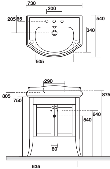
7361 Mobile chiuso laccato nero//bianco lucido per lavabo 69 Bright-black or white cabinet for washbasin 69 laquer finish
