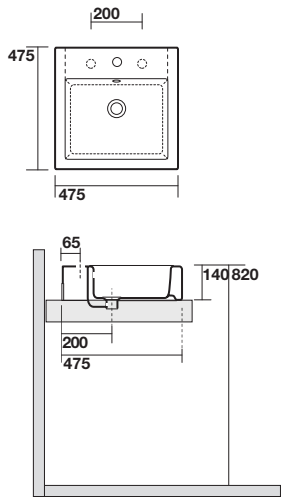
7740 “GIADA” Lavabo incasso “GIADA” Inset basin
