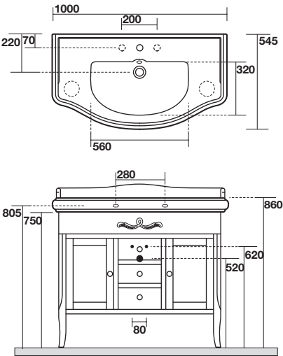
7363 Mobile cassetto laccato nero lucido//bianco lucido per lavabo 100 Bright-black or white draw unit for washbasin 100 laquer finish
