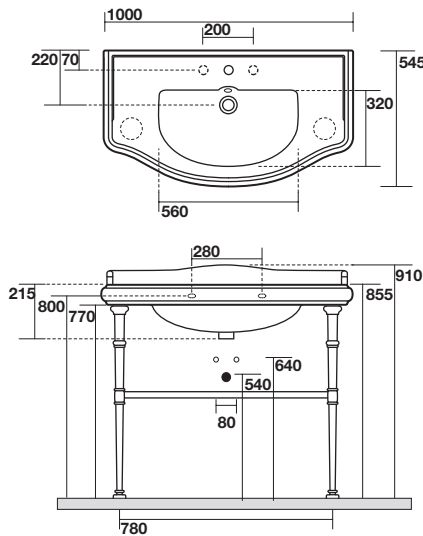
1050 consolle100 monoforo (tre fori a richiesta) One hole console 100 (three holes on demand) 1079 Supporto in ceramica completo di staffe Ceramic support w/metal bracket
