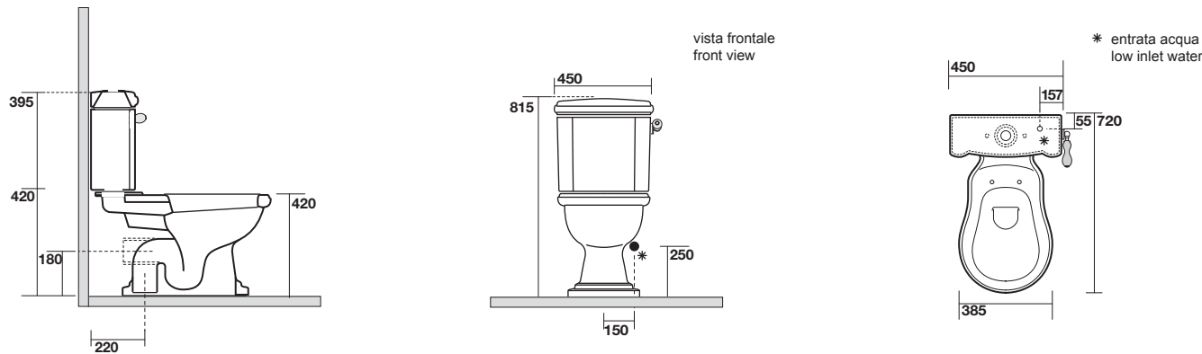
1012 vaso monoblocco scarico suolo “S” Close couped wc pan floor outlet 1013 vaso monoblocco scarico parete “P” Close couped wc pan wall outlet 1071 Cassetta monoblocco scarico leva laterale Close coupled cistern for lateral handle
